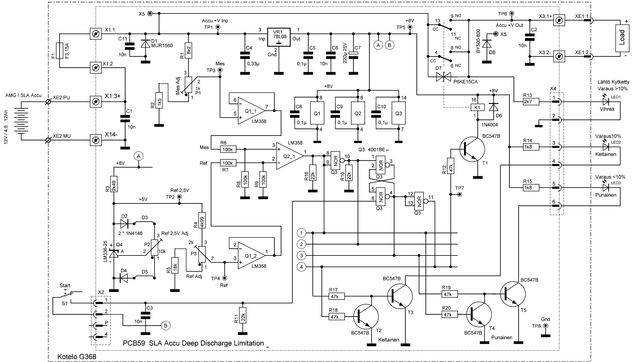
PCB59 SLA Accu Deep Discharge Limitation Connection Diagram
