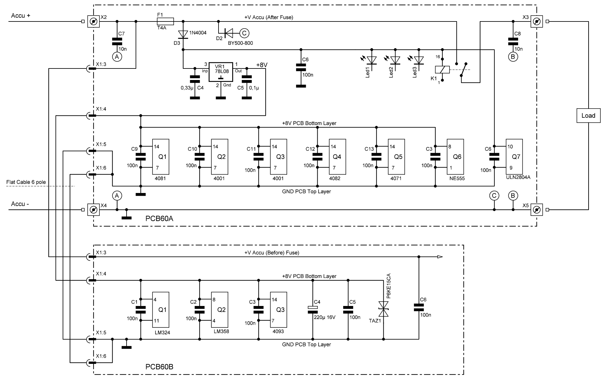
Pb Accu Deep Discharge Limitation v2 PCB60A_B Voltage Supply Logic and Analogue Sections
